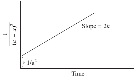
Fig. 1.6 Third order plot.
