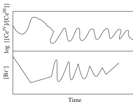
Fig. 5.2 Periodic behaviour in [\text{Br}^-] and [\text{Ce}^{\text{IV}}]/[\text{Ce}^{\text{III}}] in Belousov reaction.
