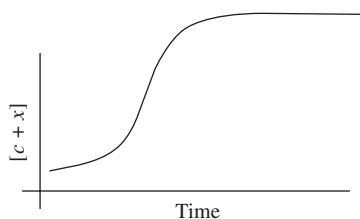
Fig. 1.5 Plot of (c + x) versus time.
