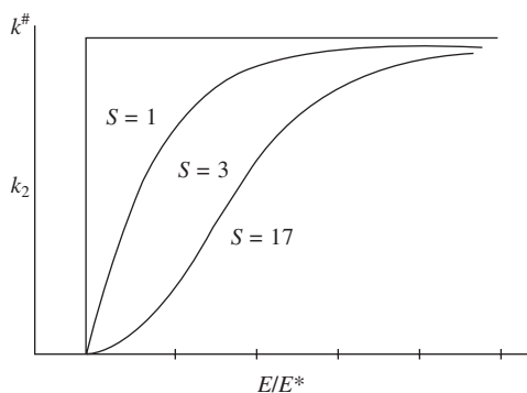
Fig. 4.11 Variation of k_2 with E/E^* .
