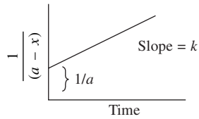
Fig. 1.4 Second order plot.
