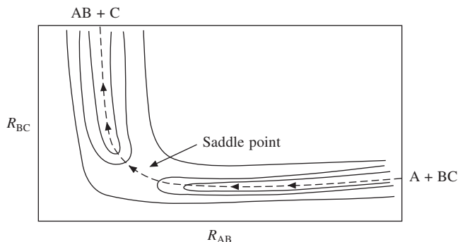
Fig. 2.6 Potential energy contour diagram for a thermoneutral reaction. Dashed line is the minimum energy path and the arrows indicate the direction of reaction.
