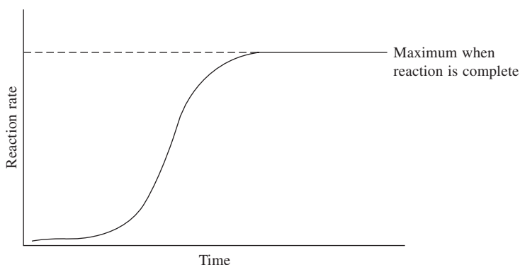
Fig. 6.1 Rate versus time plot for an autocatalytic reaction.
