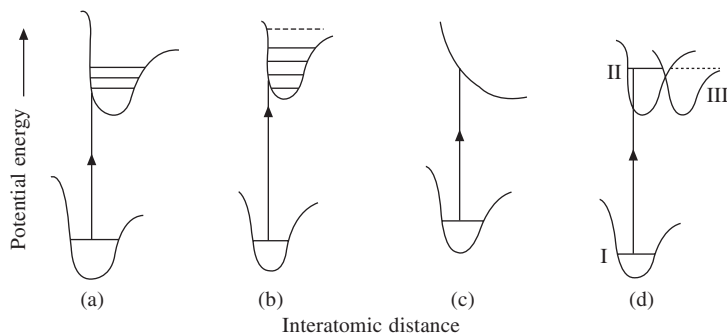
Fig. 5.1 Potential energy curves showing processes that can occur on absorption of radiation.
