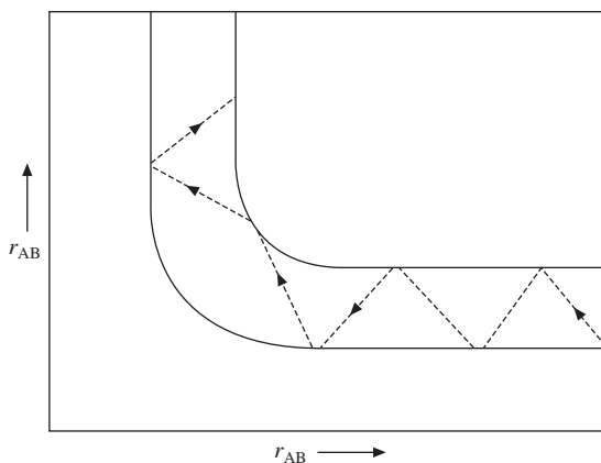
Fig. 9.32 A trajectory showing cutting the corner.
