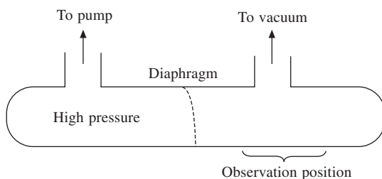
Fig. 7.4 Shock tube.
