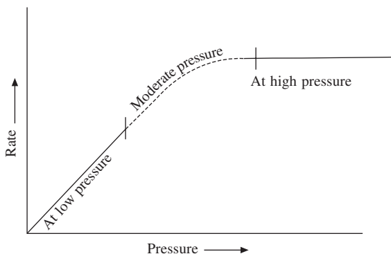
Fig. 6.8 Rate-pressure relationship for dissociation of single reactant on solid surface.
