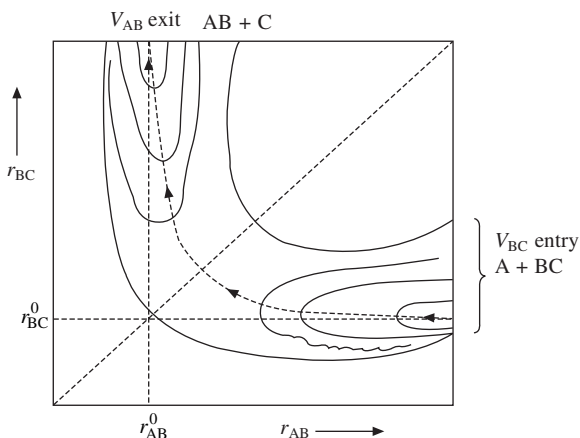
Fig. 9.12 PE contours for A + BC \rightarrow AB + C reaction.
