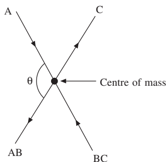
Fig. 9.35 Direction of motion of reactants and products relative to centre of mass (stripping mechanism).
